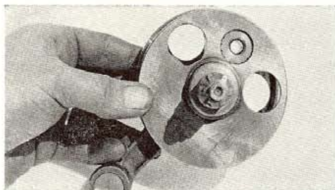
Crankshaft balance holes can be filled to bump up the primary compression—an experts job, however.
