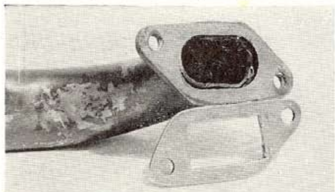
Modified exhaust gasket is shown here with exit tube before it is filled to mate cylinder flange.
