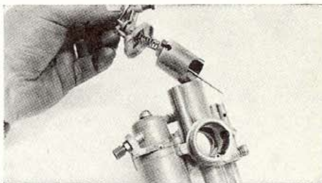
Check carb slide and make sure needle is not bent. The needle position can be experimentally raised.
