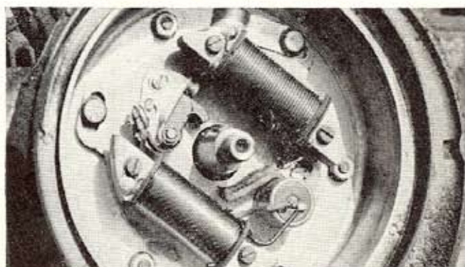
Ignition timing advance is vital. Elongated slots in breaker plate allow you to shift points further on.
